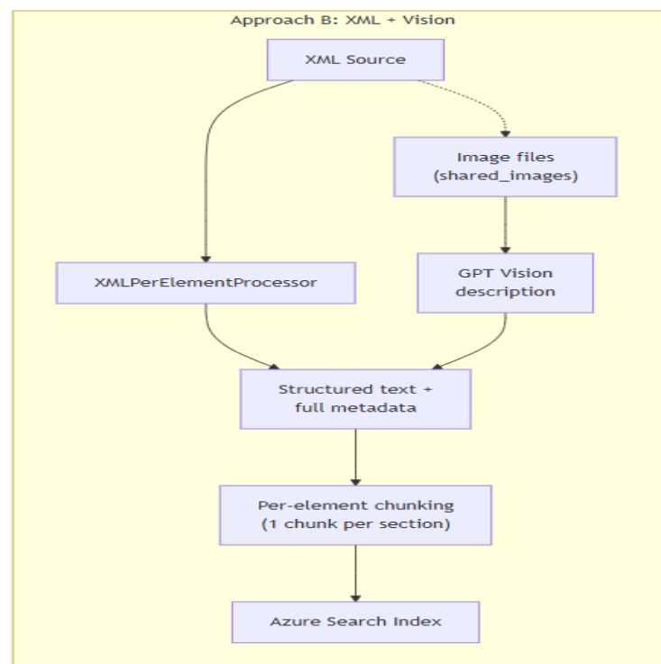
Figure 2. Configuration B (XML + Vision) processing pipeline.
