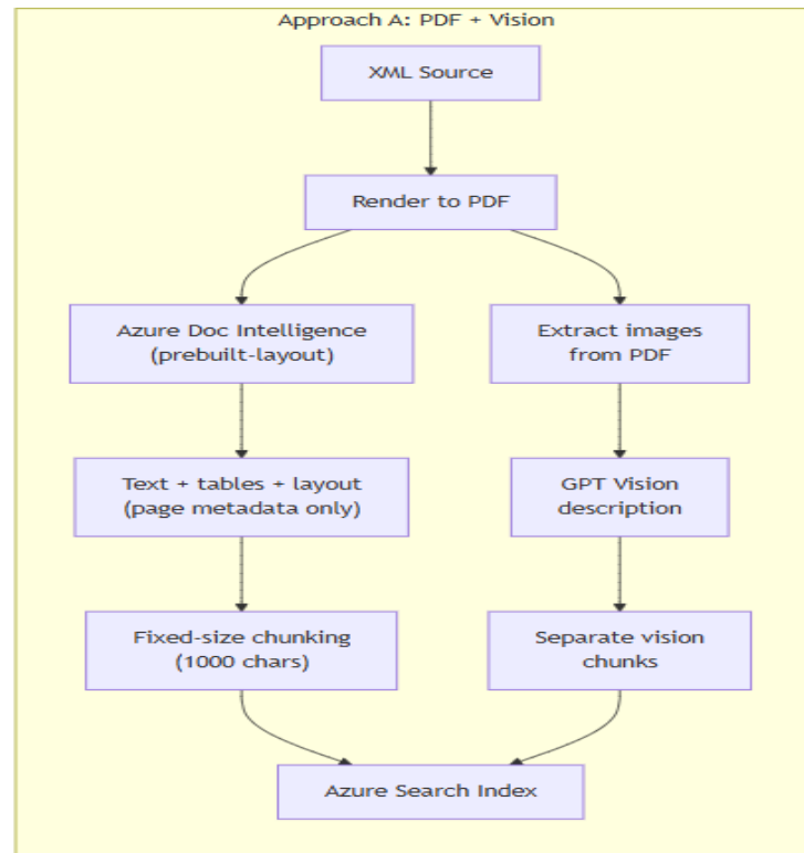
Figure 1. Configuration A (PDF + Vision) processing pipeline.
